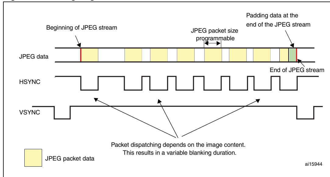
Figure 65. Timing diagram
