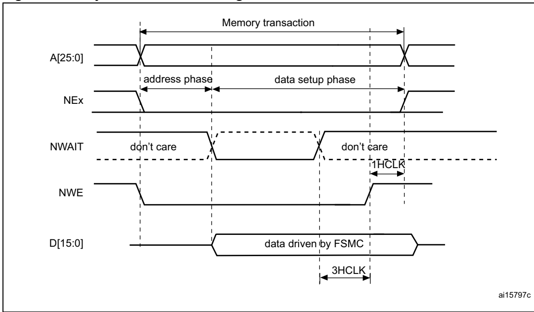
Figure 419. Asynchronous wait during a write access
