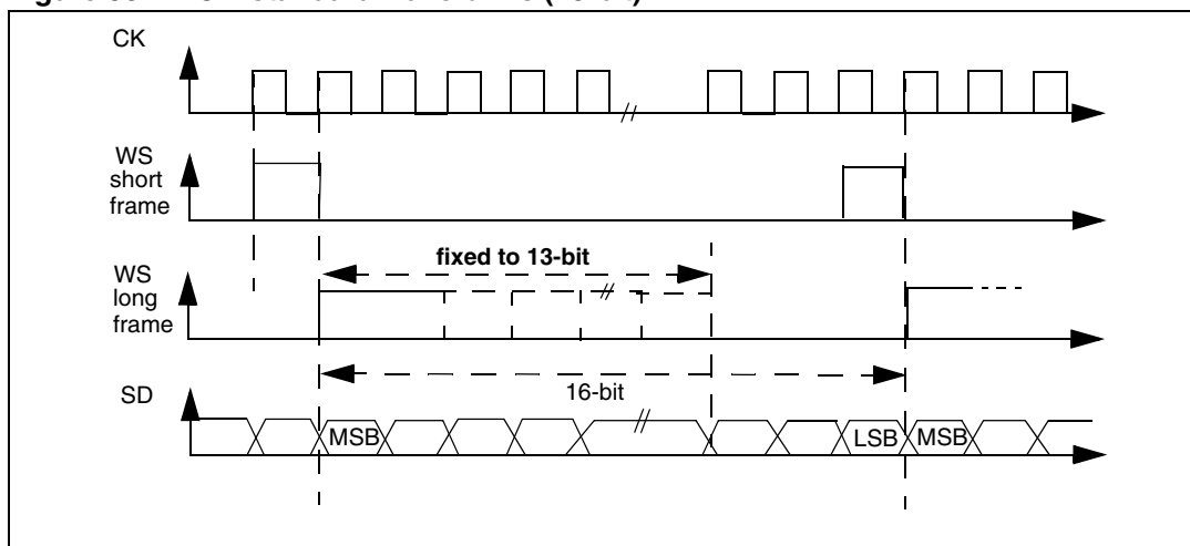
Figure 304. PCM standard waveforms (16-bit)
