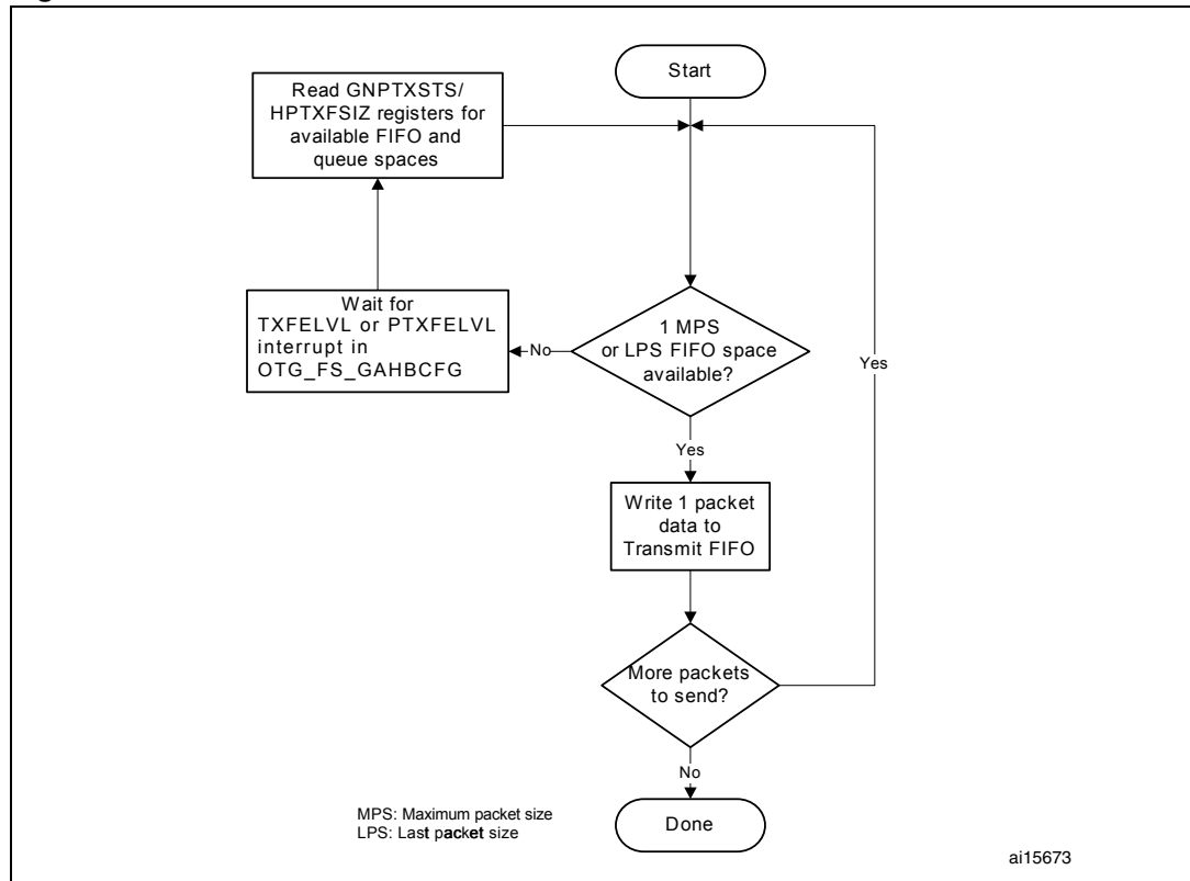
Figure 385. Transmit FIFO write task
