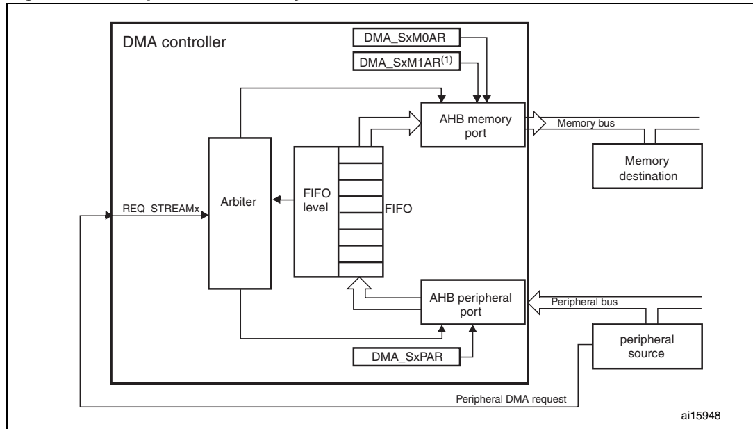
Figure 28. Peripheral-to-memory mode
