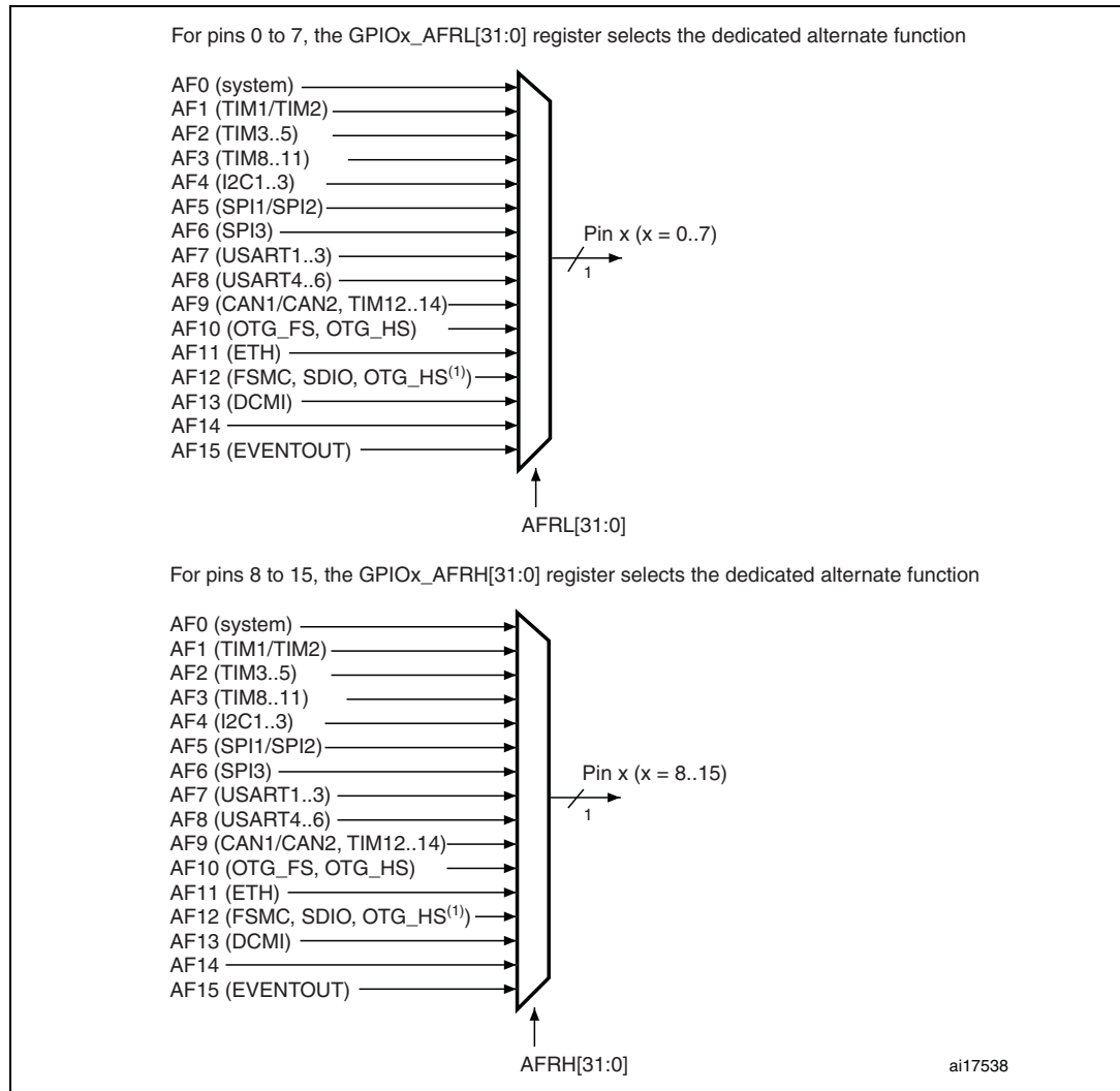
Figure 18. Selecting an alternate function on STM32F405xx/07xx and STM32F415xx/17xx
