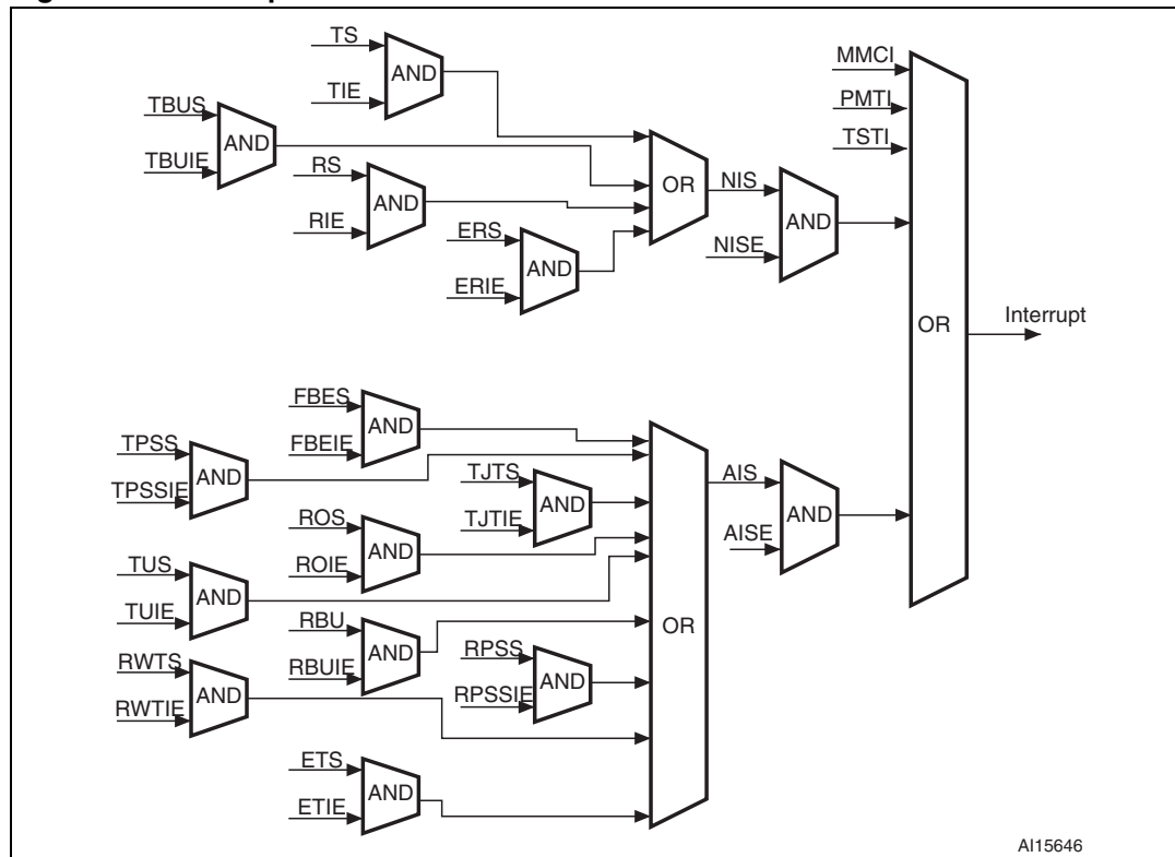
Figure 355. Interrupt scheme
