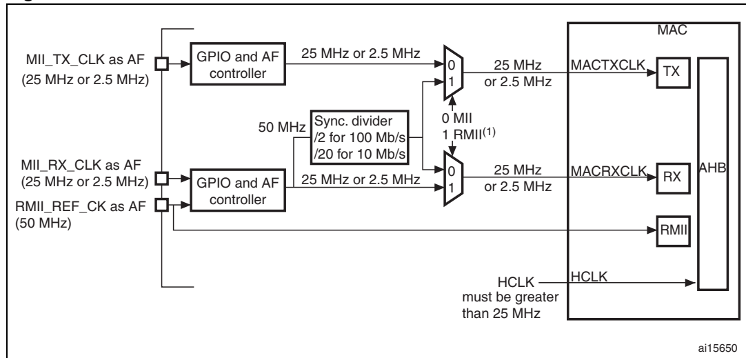
Figure 329. Clock scheme
