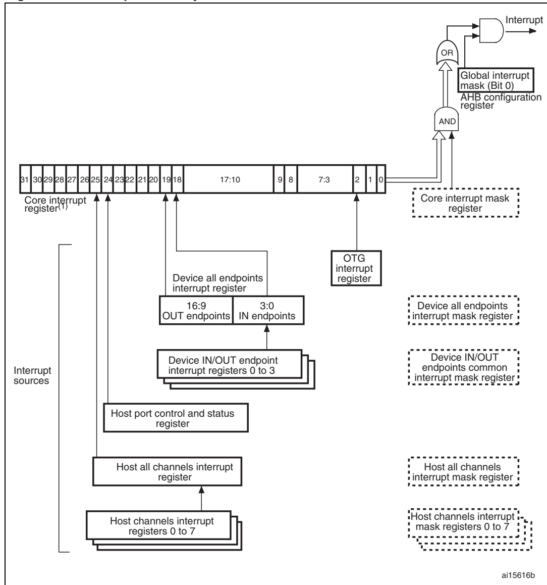
Figure 365. Interrupt hierarchy
