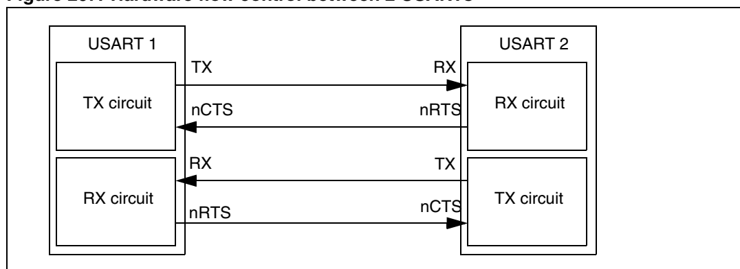
Figure 267. Hardware flow control between 2 USARTs
