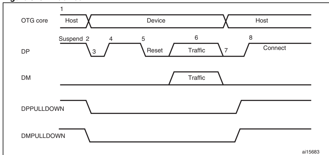
Figure 379. A-device HNP
