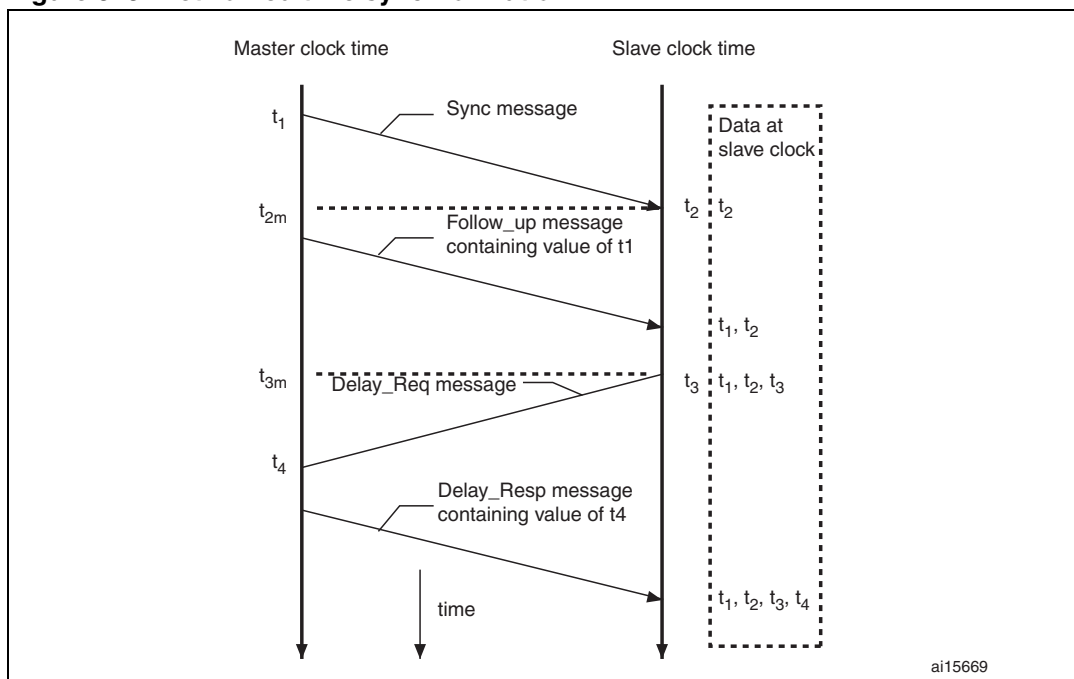
Figure 343. Networked time synchronization
