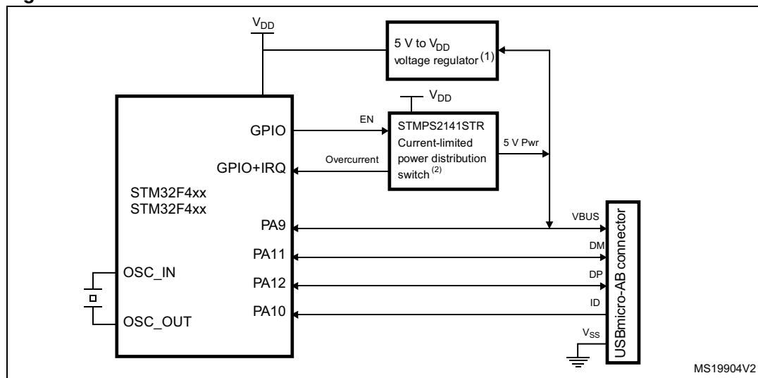
Figure 358. OTG A-B device connection
