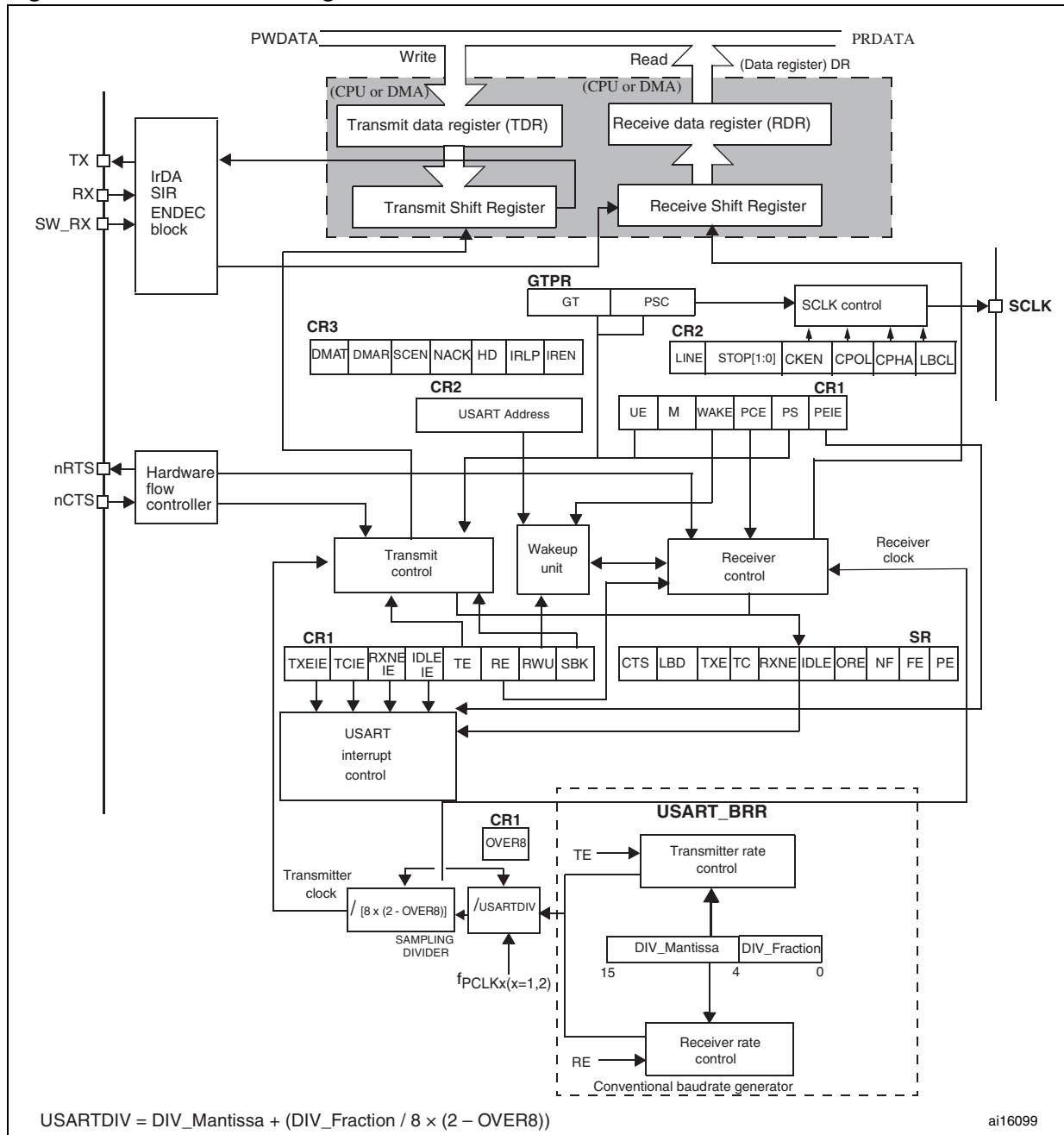
Figure 246. USART block diagram
