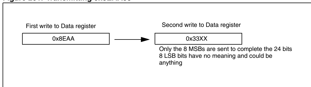
Figure 291. Transmitting 0x8EAA33
