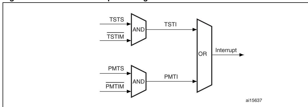
Figure 341. MAC core interrupt masking scheme
