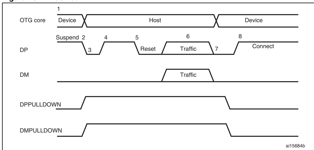
Figure 402. B-device HNP
