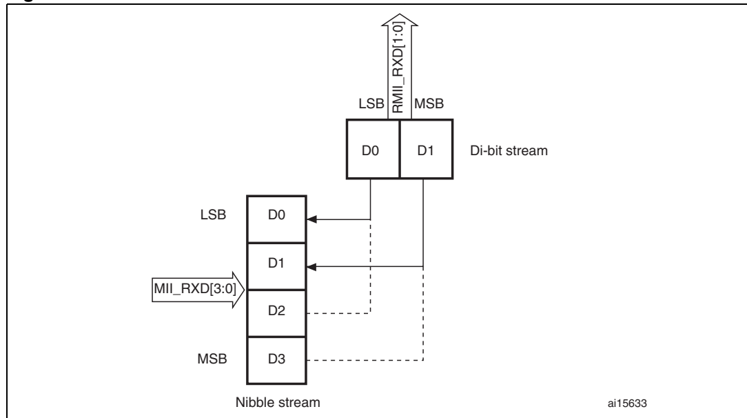
Figure 337. Receive bit order
