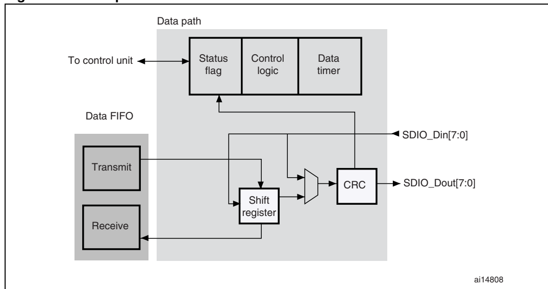
Figure 319. Data path
