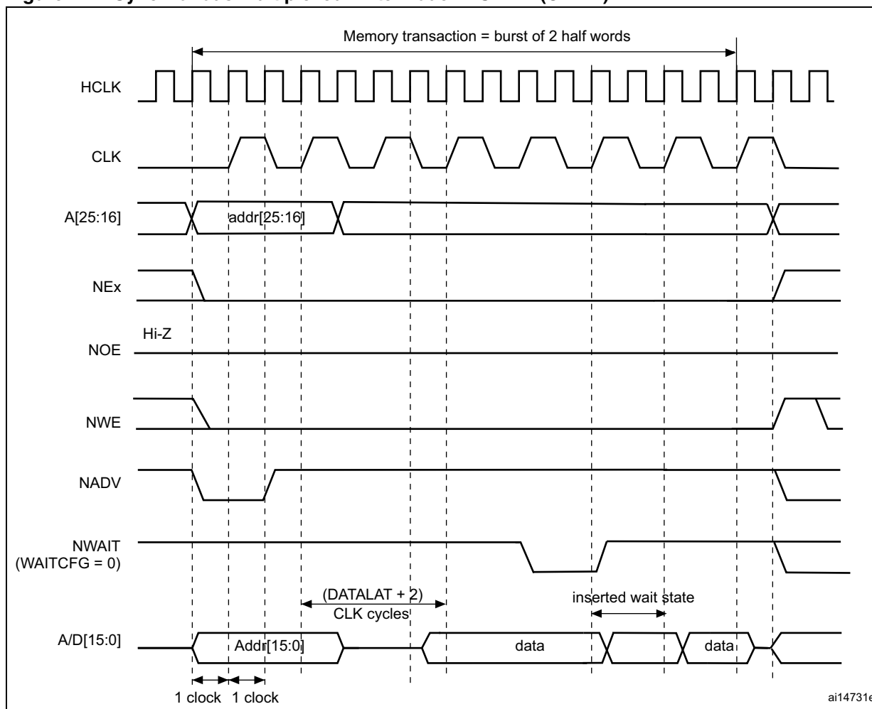
Figure 422. Synchronous multiplexed write mode - PSRAM (CRAM)
