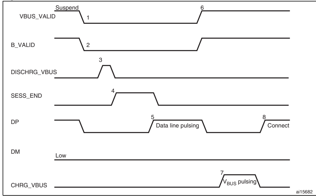
Figure 378. B-device SRP
