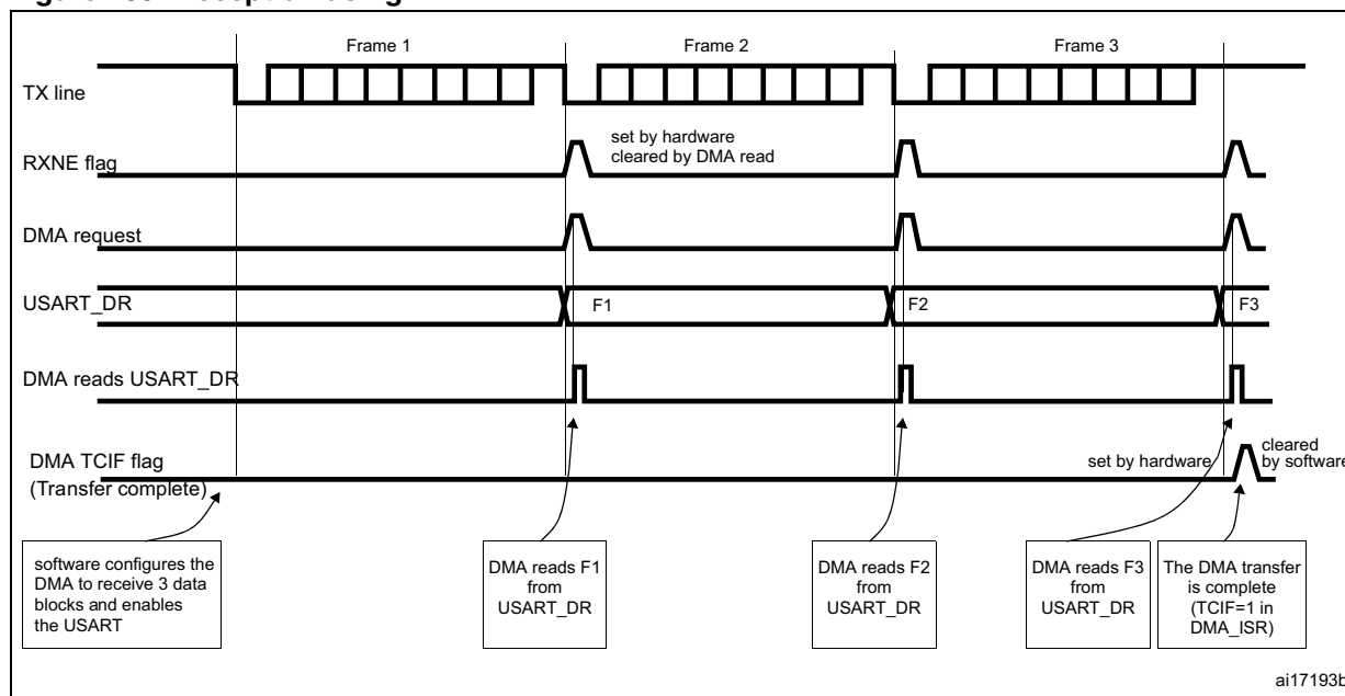
Figure 266. Reception using DMA
