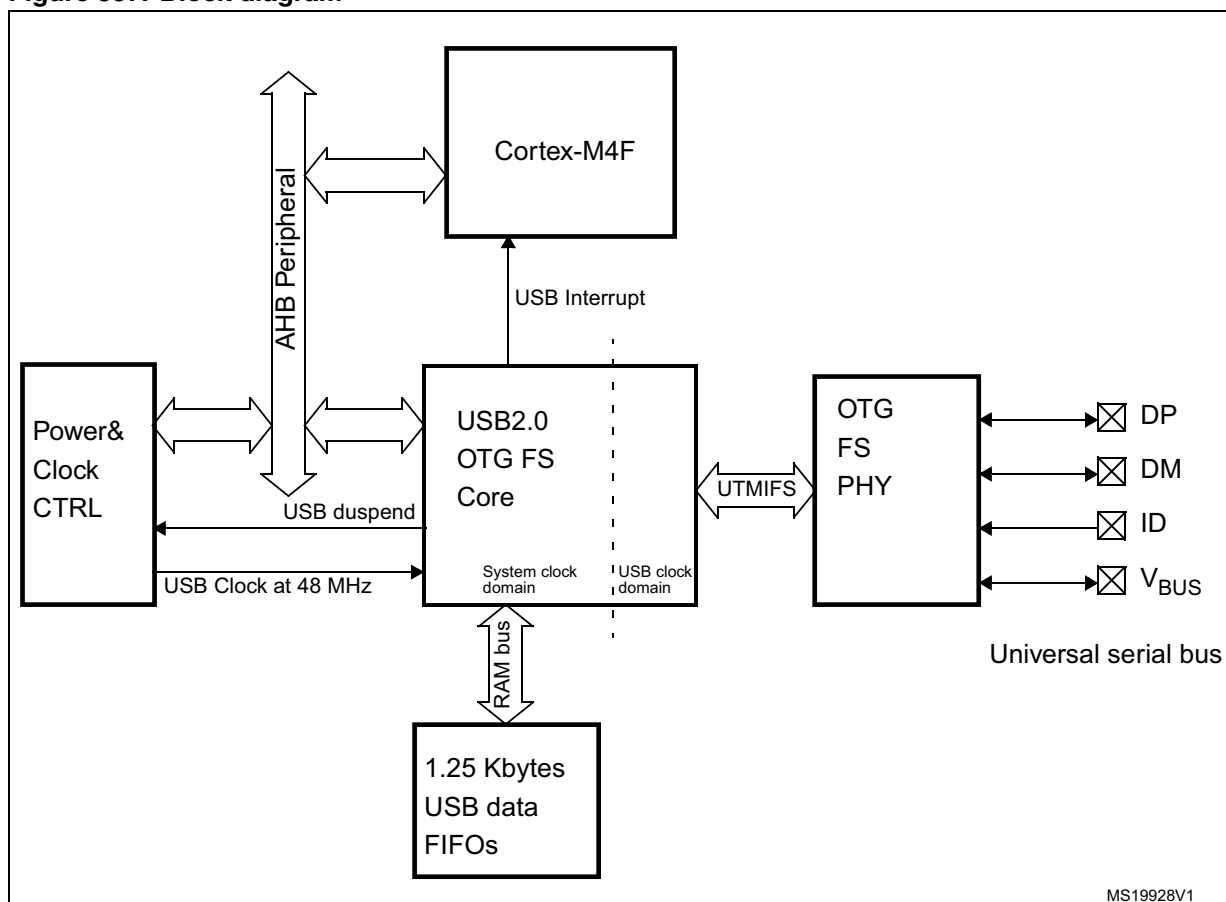
Figure 357. Block diagram
