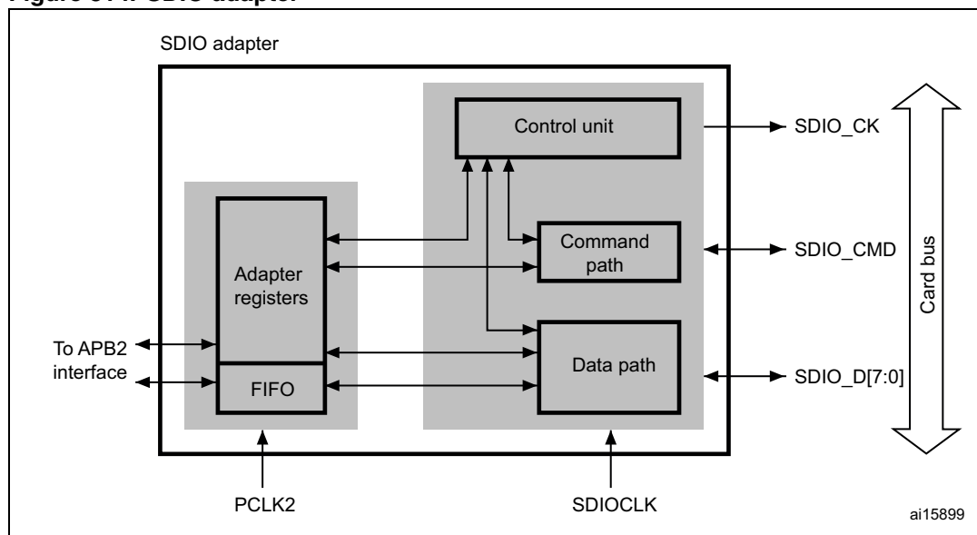
Figure 314. SDIO adapter
