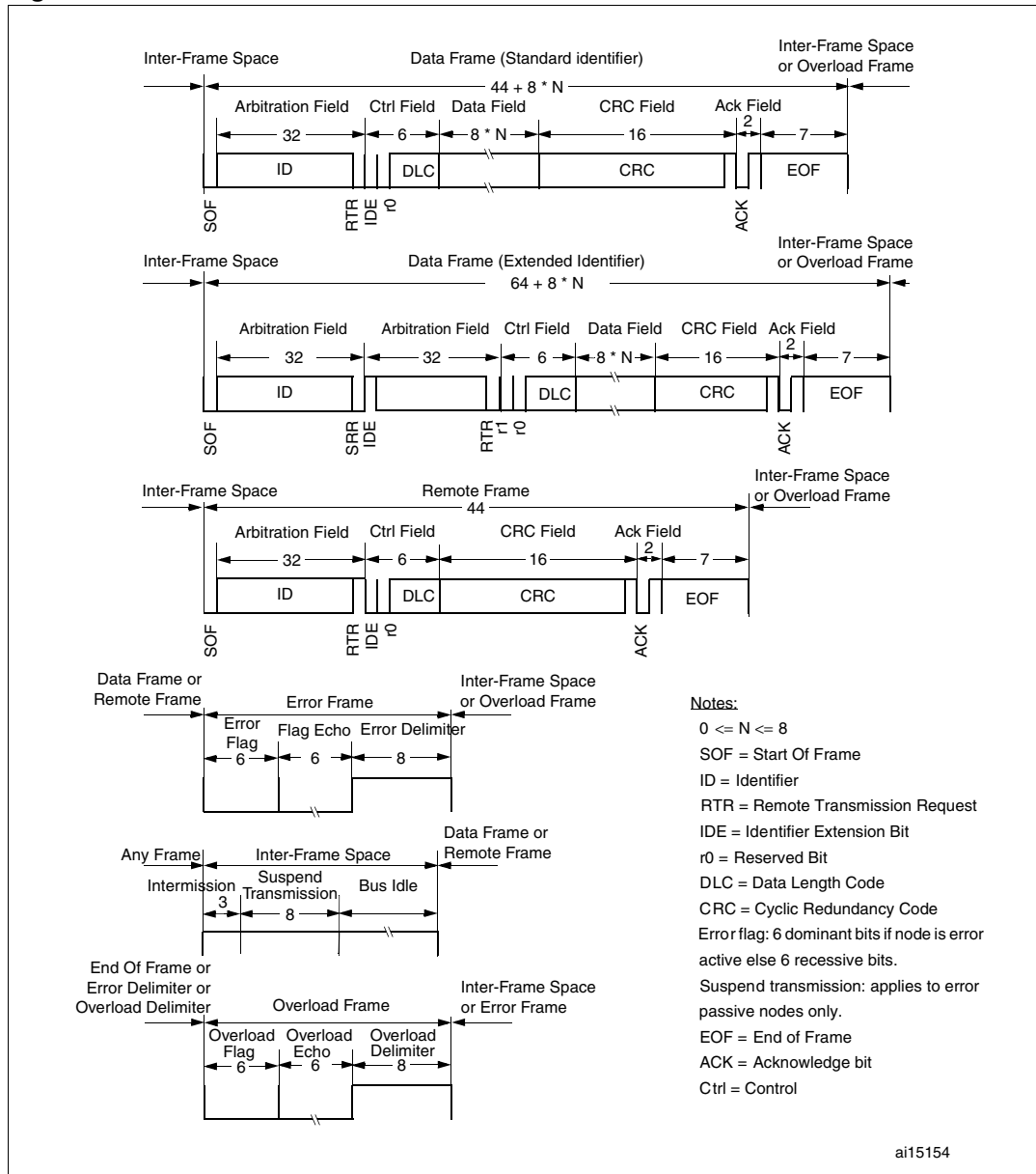
Figure 236. CAN frames
