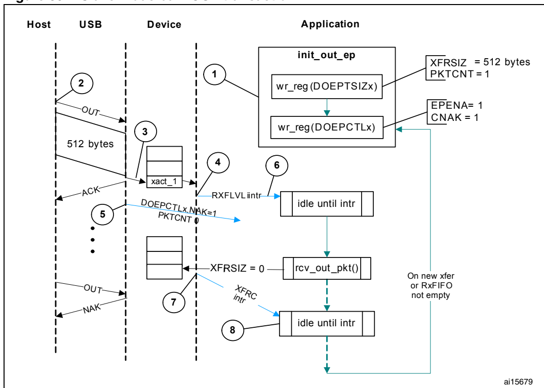
Figure 397. Slave mode bulk OUT transaction
