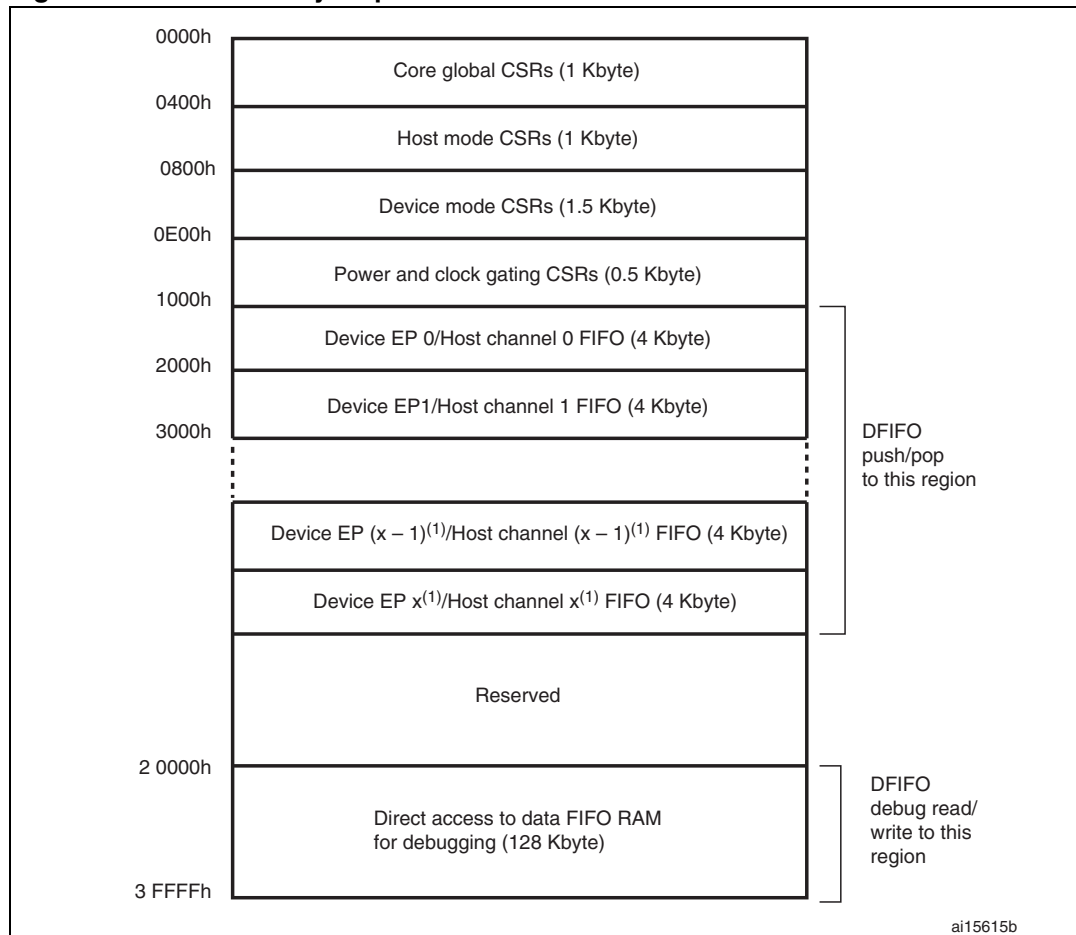
Figure 384. CSR memory map
