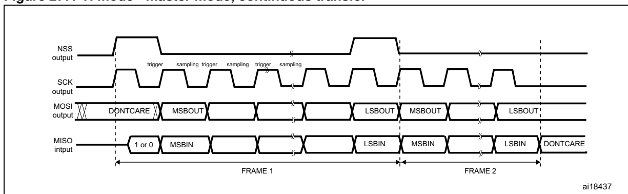
Figure 277. TI mode - master mode, continuous transfer
