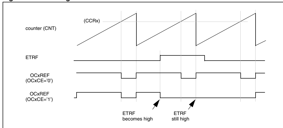
Figure 109. Clearing TIMx OCxREF
