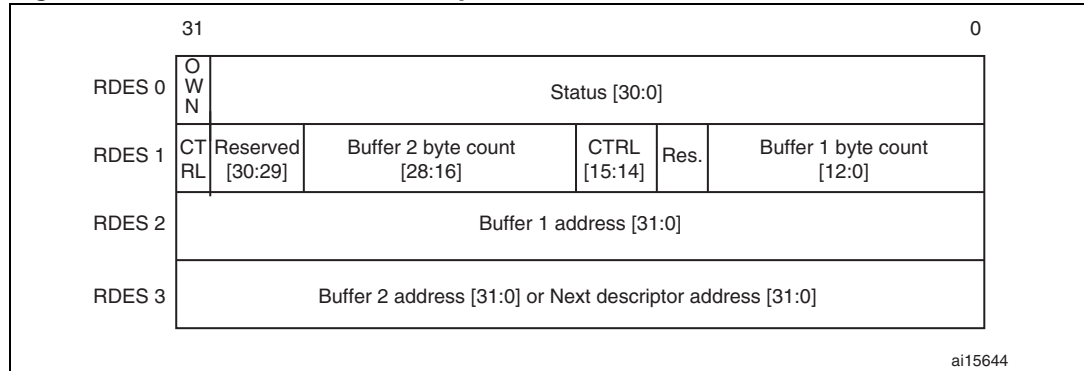
Figure 353. Normal Rx DMA descriptor structure
