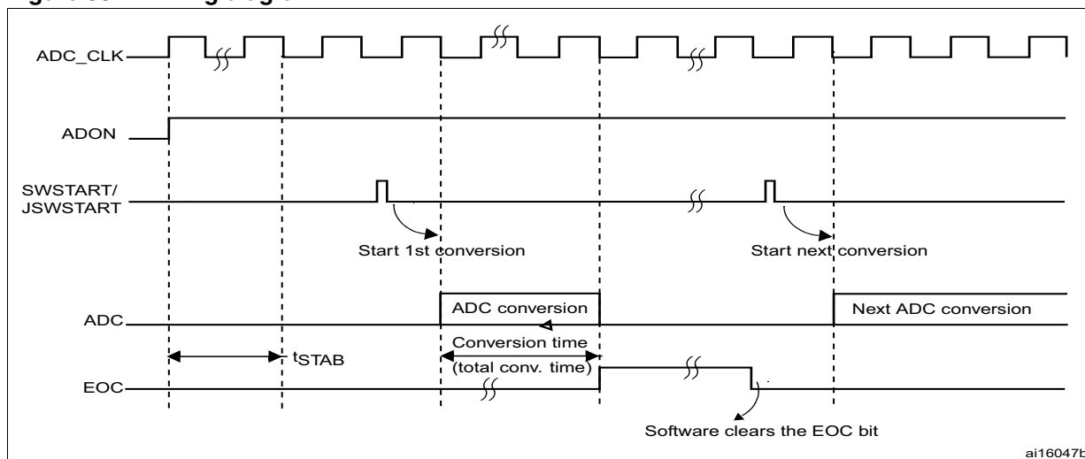
Figure 35. Timing diagram
