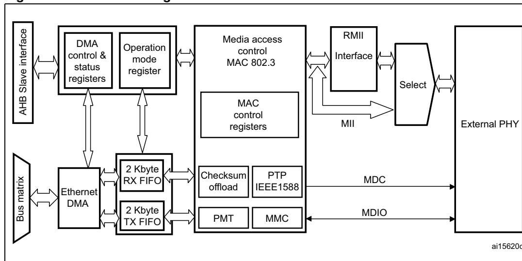
Figure 321. ETH block diagram
