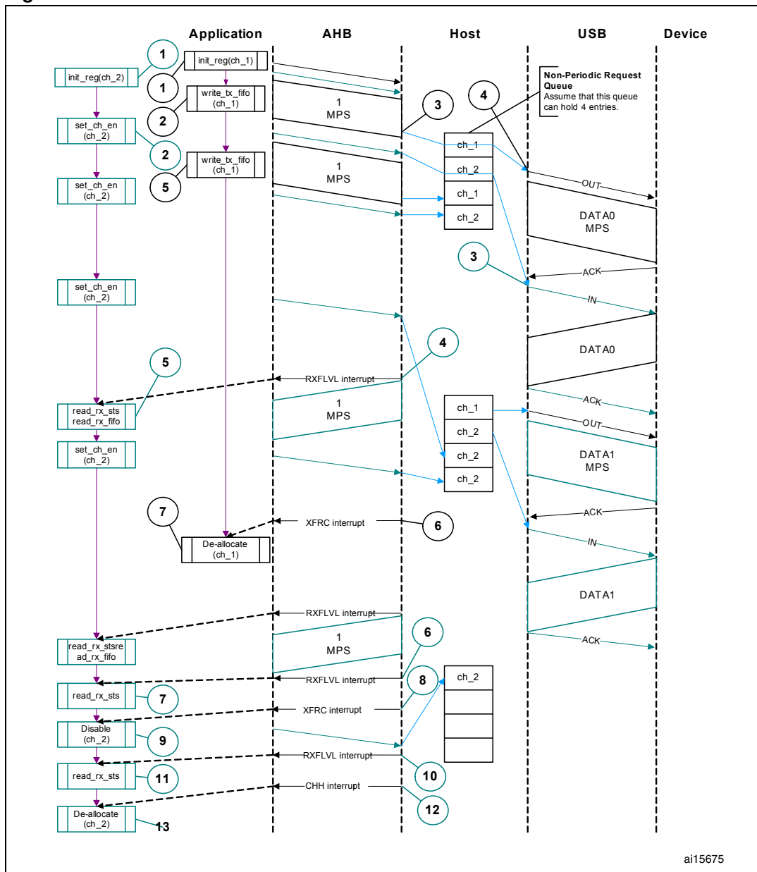
Figure 369. Normal bulk/control OUT/SETUP and bulk/control IN transactions
