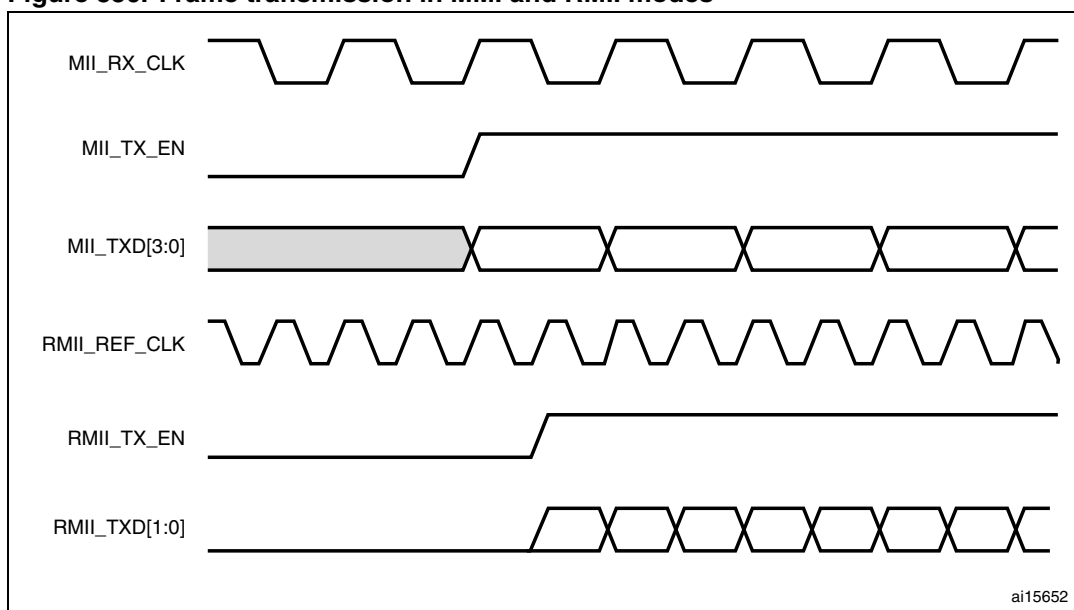
Figure 336. Frame transmission in MII and RMII modes
