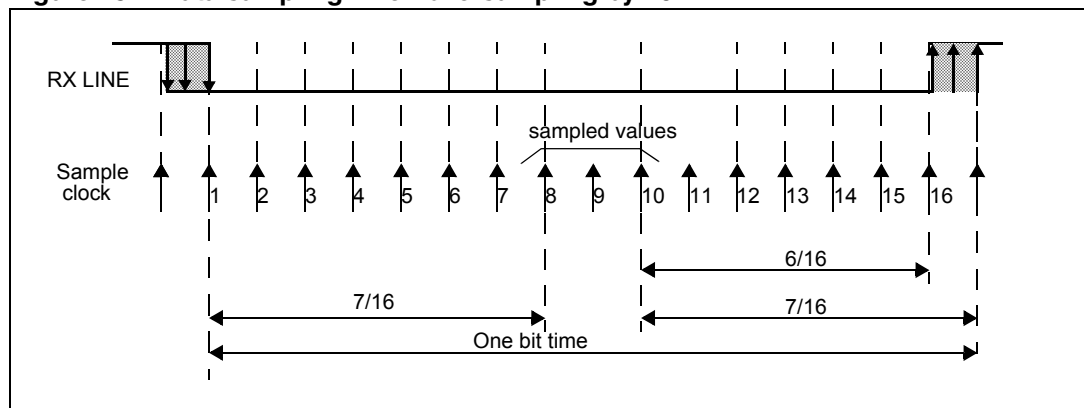
Figure 252. Data sampling when oversampling by 8
