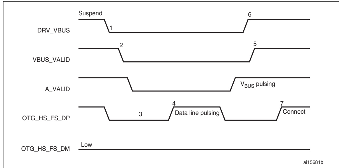
Figure 399. A-device SRP
