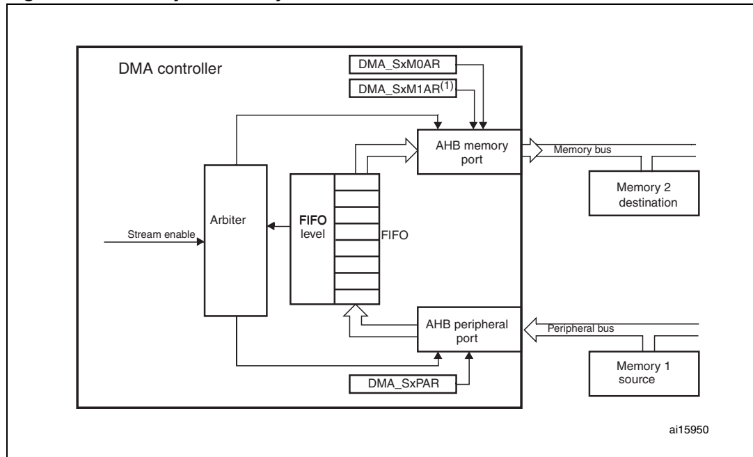
Figure 30. Memory-to-memory mode
