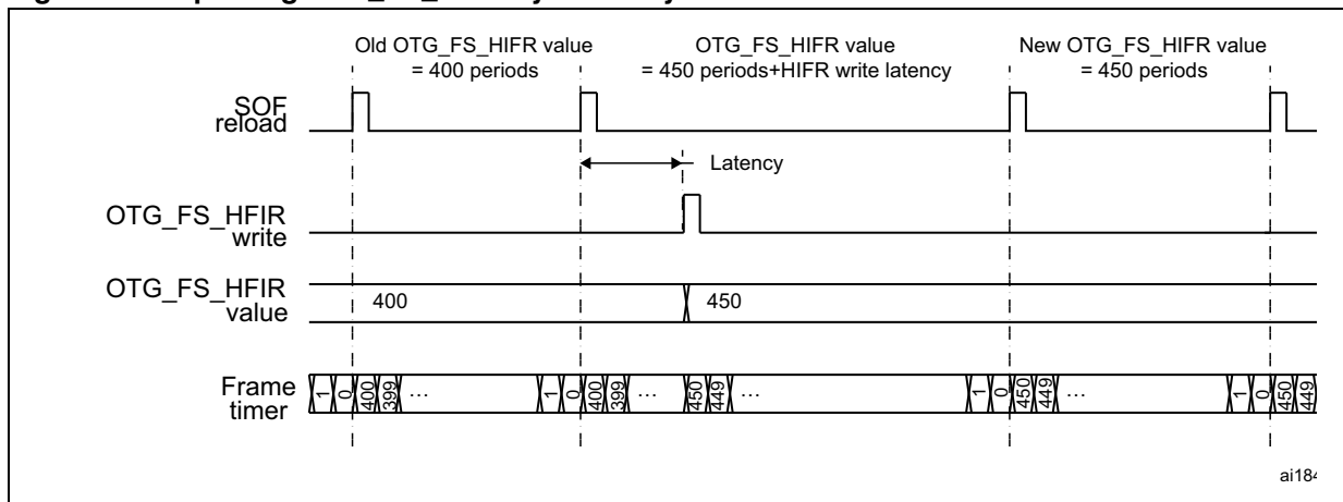
Figure 362. Updating OTG_FS_HFIR dynamically
