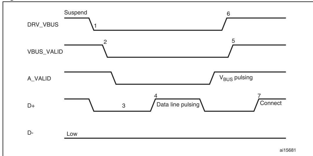
Figure 377. A-device SRP
